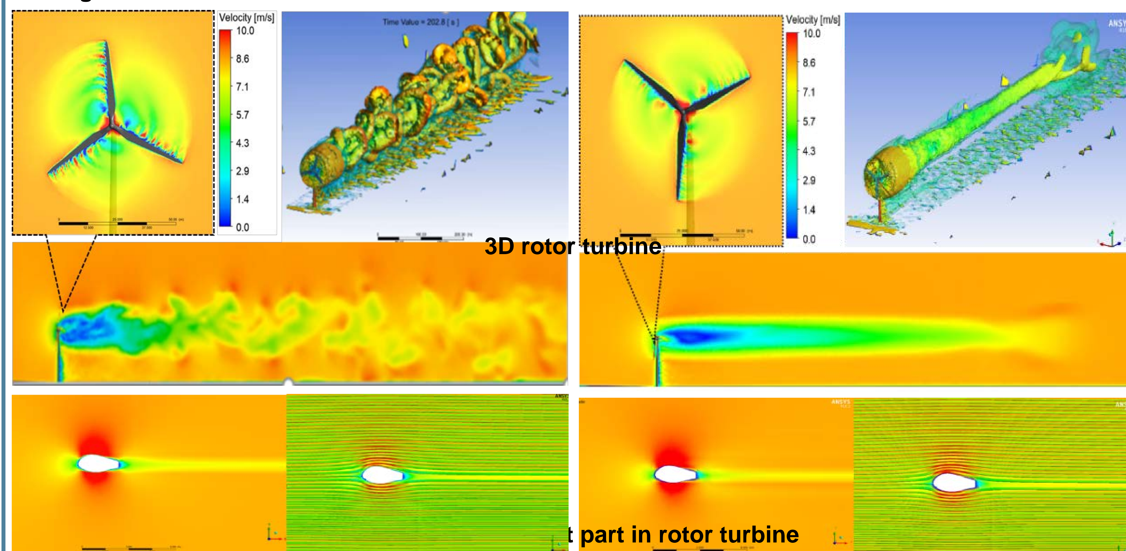
Fig. 3. CFD simulation results for LES model and RANS model.
