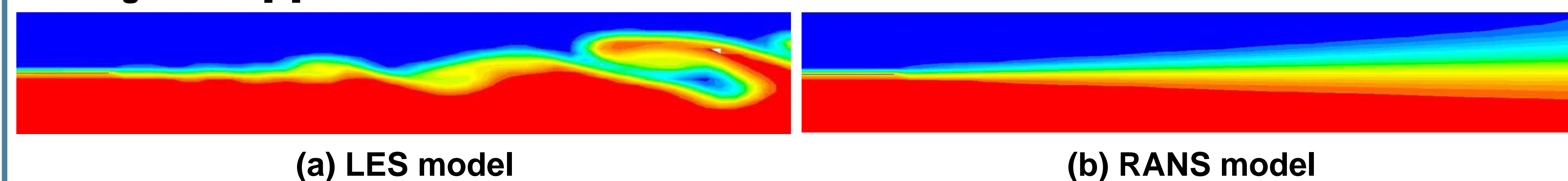
Fig. 1. Major turbulent models in CFD simulation (ANSYS Fluent).
