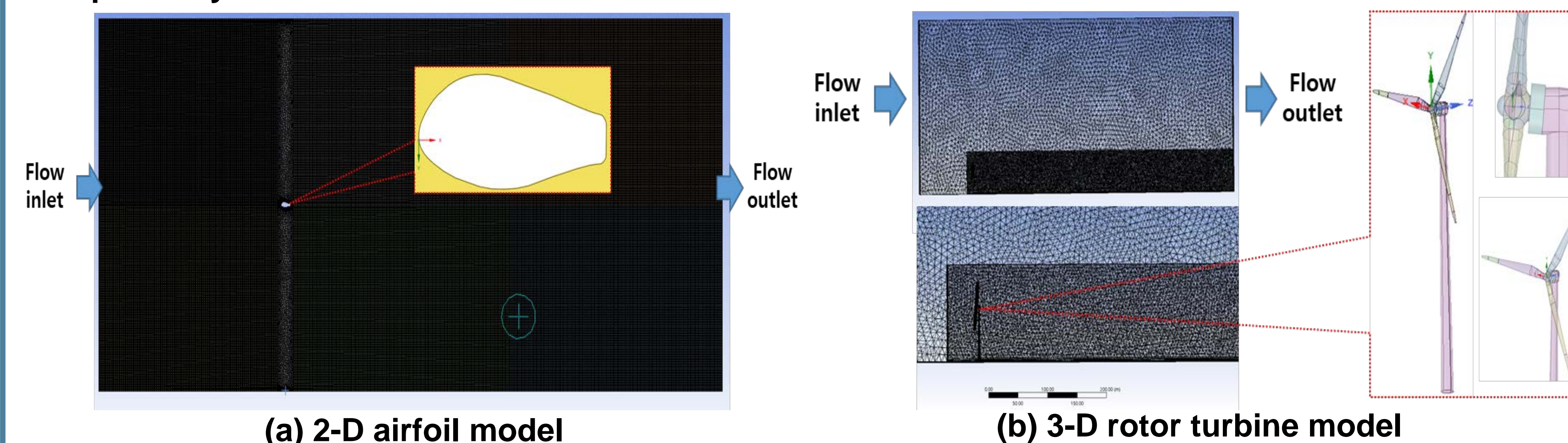
Fig. 2. Numerical schemes of 2-D and 3-D models.
